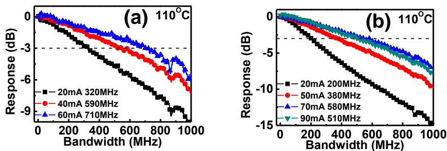
Fig. 4. (a) The measured bias dependent E-O frequency responses of the (a) 47 \mu\text{m} device and (b) 75 \mu\text{m} device under 110 ^{\circ}\text{C} operation.
