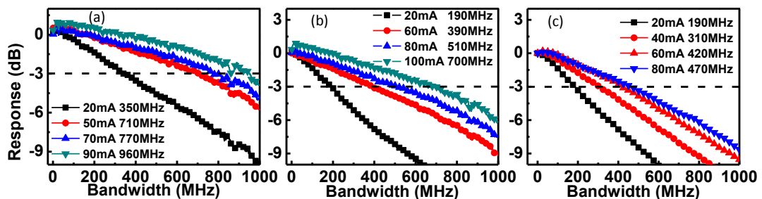
Fig. 3. (a) The measured bias dependent E-O frequency responses of the (a) 47 \mu\text{m} device, (b) 75 \mu\text{m} device, and (c) 75 \mu\text{m} device after TO-Can packaging under RT operation.
