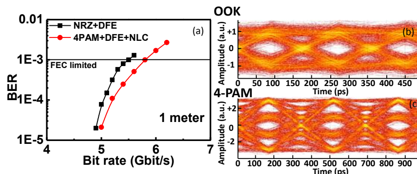
Fig. 5. (a) The measured BER values versus bit rates of an LED under NRZ and with a 4-PAM modulation format over 1 m SI-POF. (b) NRZ and (c) 4-PAM eye patterns at 5.5 and 5.8 Gbit/s, respectively.
