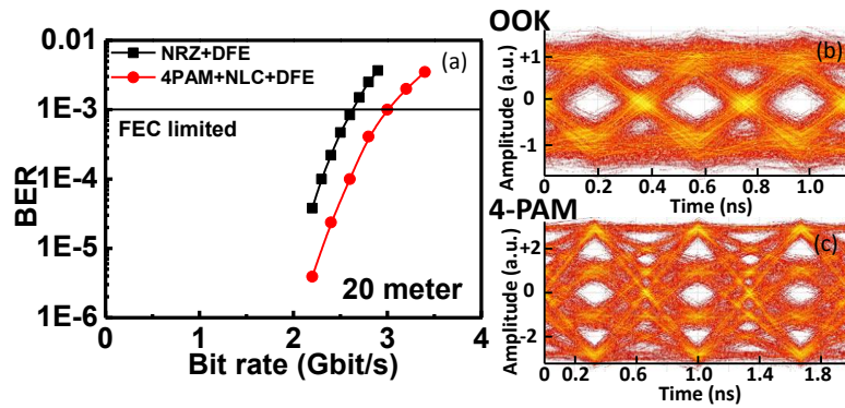
Fig. 6. (a) The measured BER values versus bit rates of an LED under NRZ and 4-PAM modulation format over 20 m SI-POF. (b) NRZ and (c) 4-PAM eye patterns at 2.6 and 3 Gbit/s, respectively.
