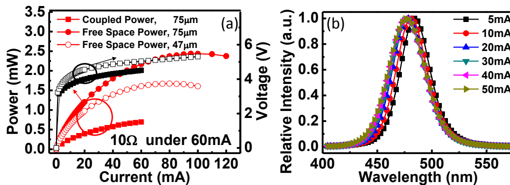
Fig. 2. (a) The measured free-space output power, coupled power into the SI-POF, and voltage vs. bias current of devices with 75 (closed symbols) and 47 (open symbols) \mu\text{m} active diameters. The measured differential resistance of both devices is around 10 \Omega under a 60 mA bias current. (b) Measured bias dependent EL spectra of a device with a 75 \mu\text{m} active diameter.
