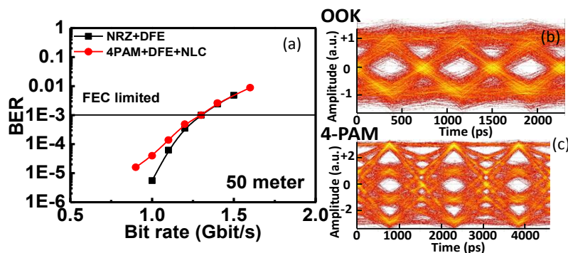
Fig. 7. (a) The measured BER values versus bit rates of an LED under NRZ and 4-PAM modulation format over 50 m SI-POF. (b) NRZ and (c) 4-PAM eye patterns at the same data rate as 1.3 Gbit/sec.
